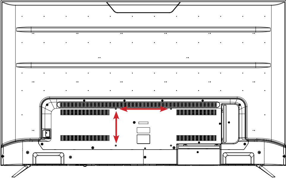
BACK OF TV VESA PATTERN: 300 (w) x 200 (h) mm
